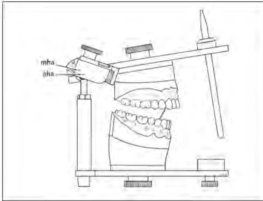
Fig 3-5 The dissimilarity between the hinge axis of the full-size semi-adjustable articulator (aha) and the mandibular hinge axis (mha) will cause a slight discrepancy between the arcs of closure of the articulator (dotted line) and of the mandible (solid line). (Reprinted from Hobo et al 2 with permission.)
