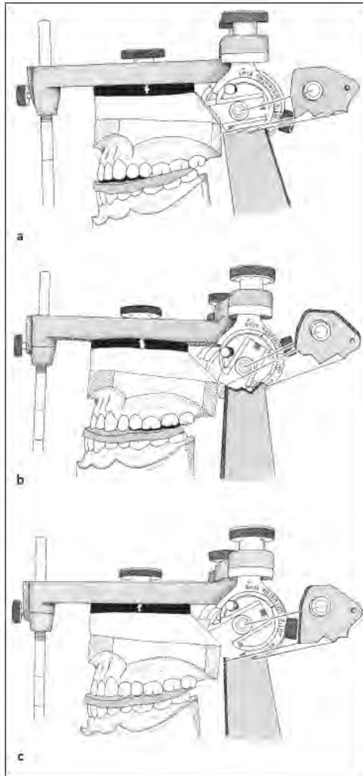
Fig 5-68 When using a protrusive interocclusal record to set the condylar guidance, the condylar inclination is rocked up and down. (a) When the angle
