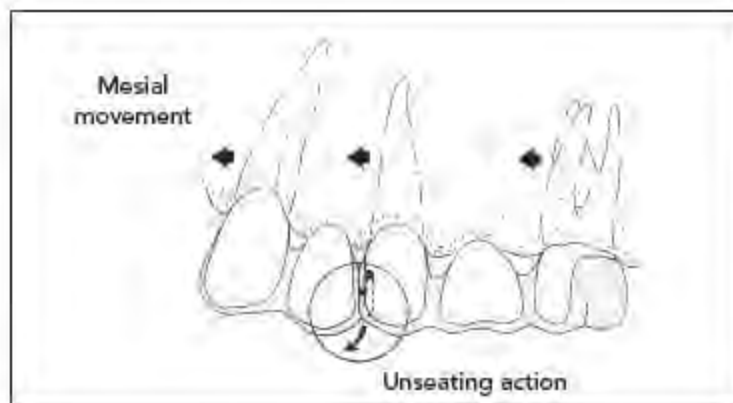
Fig 7-25 If a nonrigid connector is placed on the mesial side of the middle abutment, mesially directed movement will unseat the key. (Reprinted from Shillingburg and Fisher 19 with permission.)
