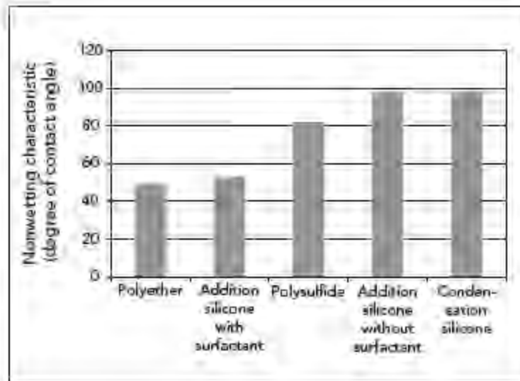
Fig 17-1 Likelihood of trapping bubbles while pouring an impression as measured by the contact angle of gypsum on their surfaces. (Based on data from McCormick et al 4 and Powers and Sakaguchi. 7 )
