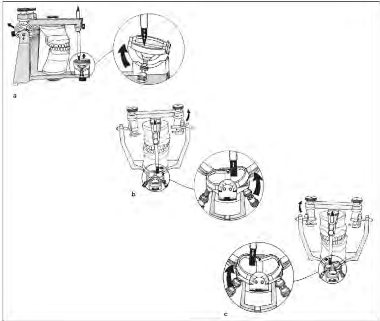
Fig 5-75 To set the mechanical incisal guide, the casts are moved into a protrusive relationship. (a) The angulation of the table is increased to contact the pin. (b) The casts are moved into a right lateral excursion, and the left wing of the incisal table is raised. (c) The casts are moved into a left lateral excursion, and the right wing of the table is lifted to complete the recording.
