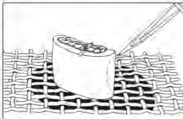
Fig 26-23 The flame is directed against the investment from all sides until it glows if the flame is left in one place for a few seconds.
