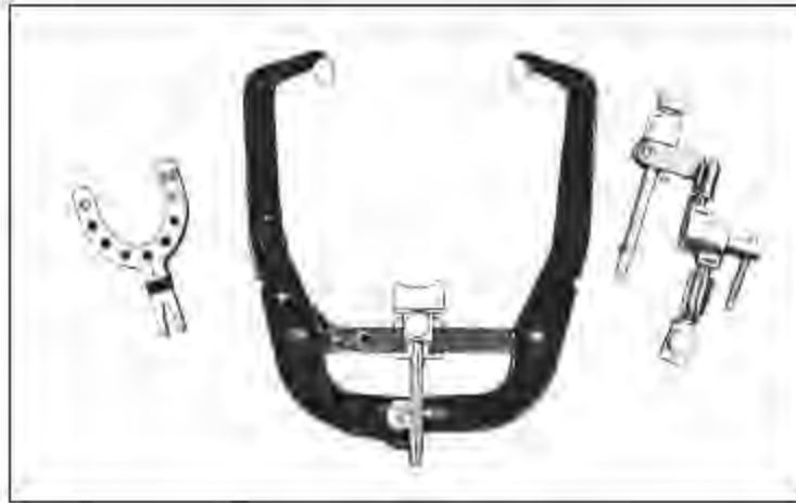
Fig 5-1 The components of a QuickMount facebow are (left to right) a bite fork, the facebow with the nasion relator, and the Quick Lock Toggle assembly.
