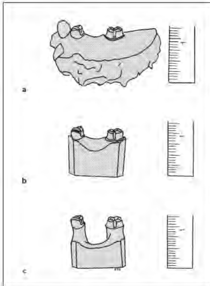
Fig 25-37 (a) An untrimmed die should measure approximately 1.25 inches
