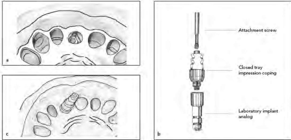
Fig 28-6 (a) Intaglio view of preliminary closed tray alginate impression. Note the detail of the impression coping in the impression material. (b) Closed tray impression coping with attachment screw and laboratory implant analog. (c) Closed tray impression coping with attached laboratory implant analog inserted into the preliminary alginate impression.
